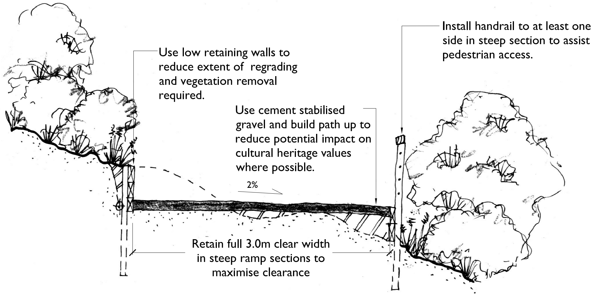
2b - STEPHENS PARADE TO 33W (SIGNPOST) BEACH CAR PARK TYPICAL CONSTRAINED TRAIL SECTION
